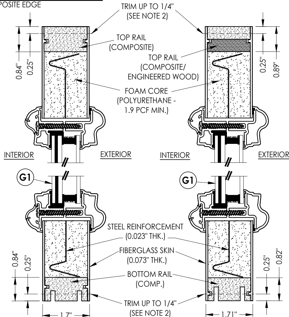
3 2 VERTICAL CROSS SECTION WOOD EDGE
