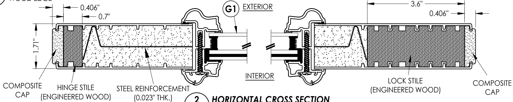
2 2 HORIZONTAL CROSS SECTION COMPOSITE EDGE
