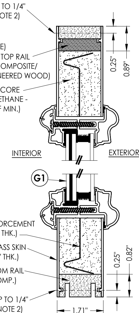
4 2 VERTICAL CROSS SECTION COMPOSITE EDGE
