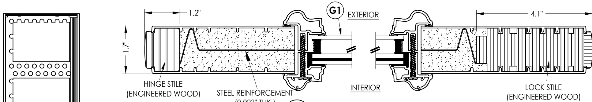
1 2 HORIZONTAL CROSS SECTION WOOD EDGE
